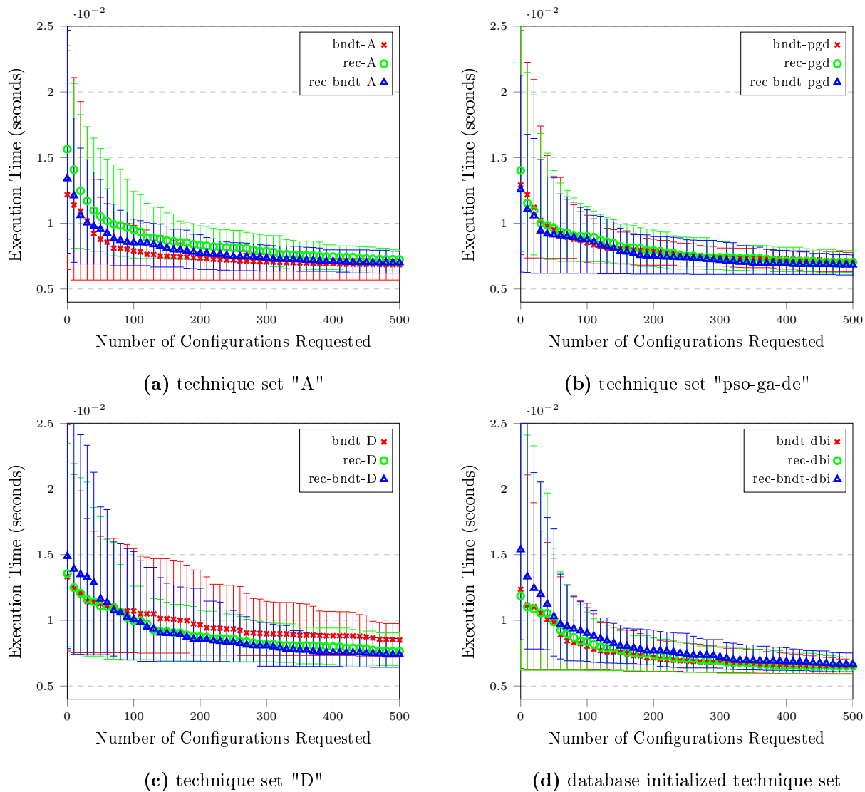
Figure 7.4: Search approach performance in Petabricks matrix approximation by initial technique set. Best execution time achieved as a function of number of configurations tested by the search approach, aggregated over 150 tuning runs. Lower execution time is better.
